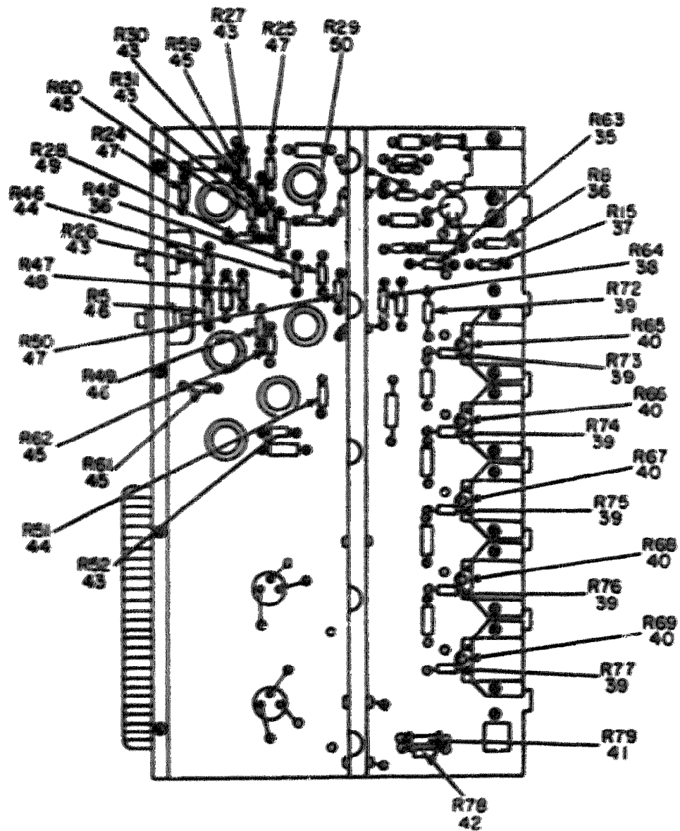
LEFT VIEW, RESISTOR LOCATION
