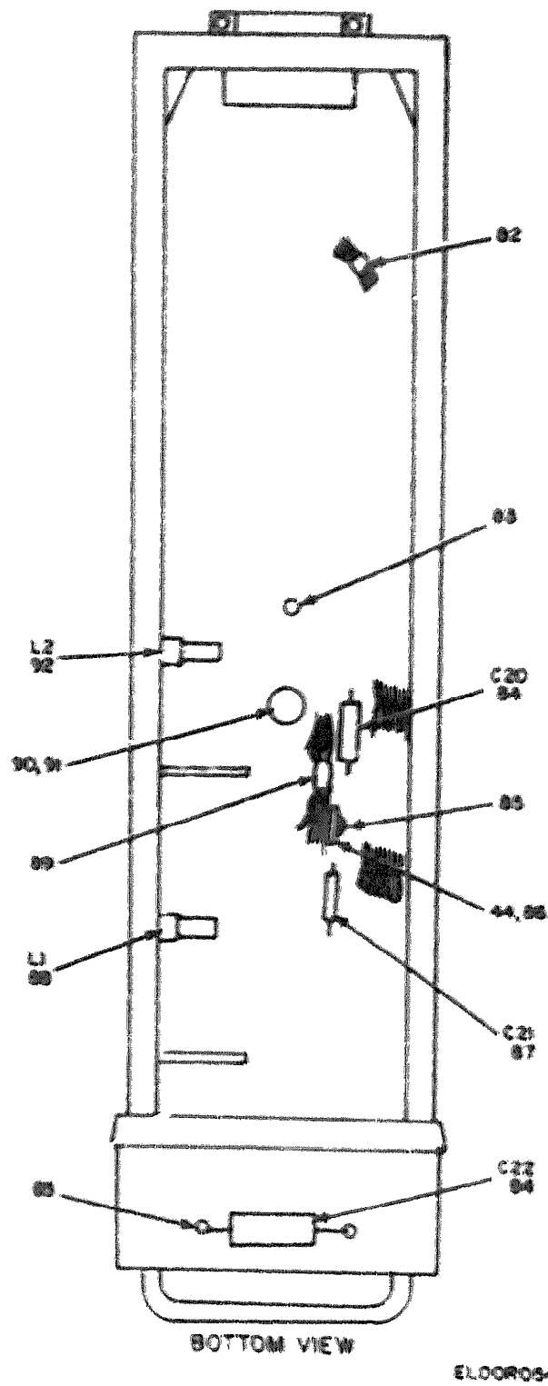
Figure 38. Synchronizer, Electrical SN-358/APN-158, Additional Parts Location (Sheet 3 of 4).
