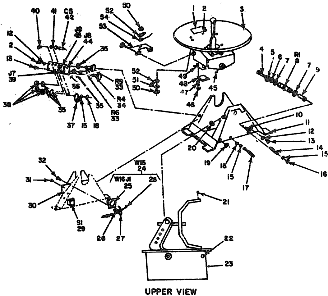
Figure 2. Antenna AS-1520/APN-158 or Antenna AS-1642/APN-158 (Sheet 1 of 2).
