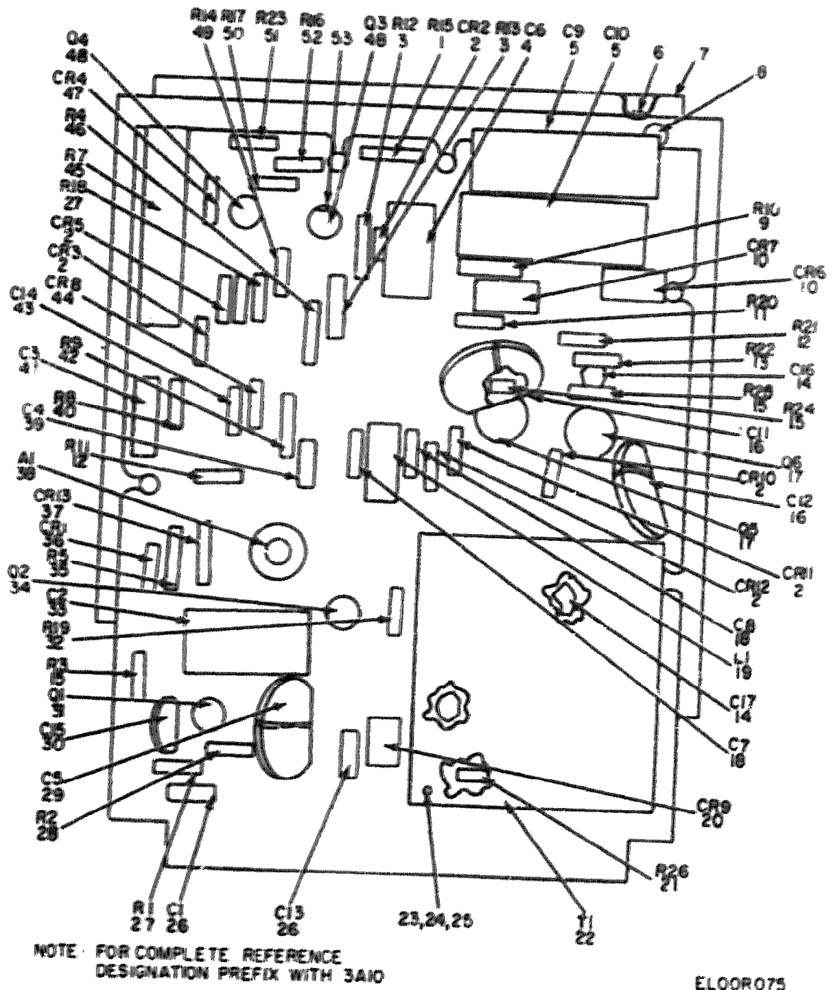
Figure 51. AFC Assembly (3A10) (772-0968-003).
