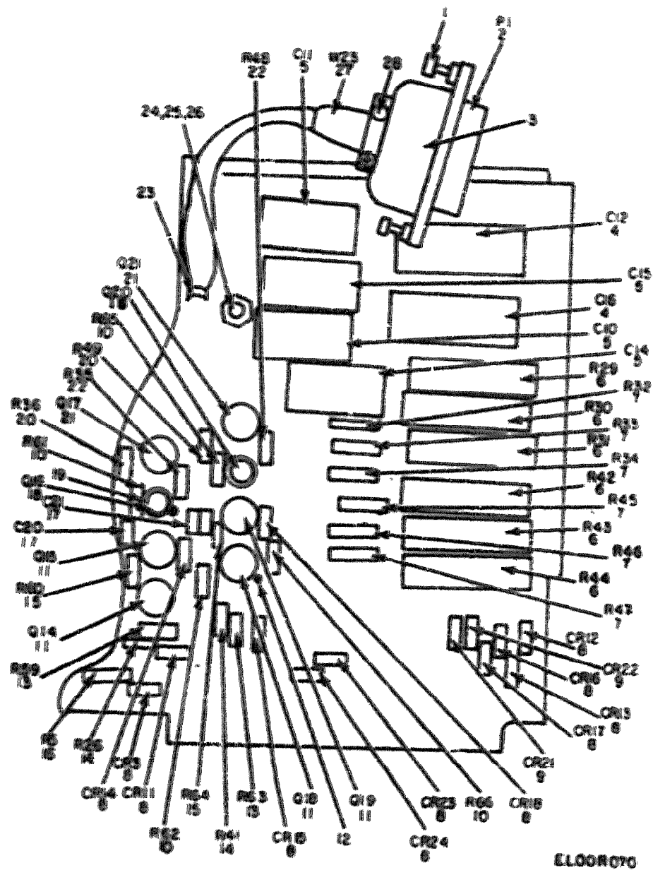
Figure 48. Generator-Amplifier, Sweep (3A7) (Sheet 1 of 3).
