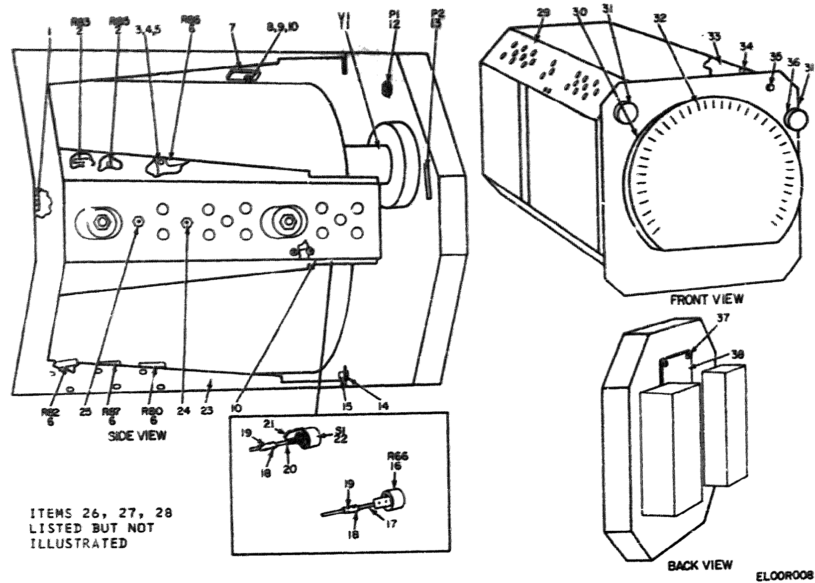
Figure 7. Indicator, Azimuth-Range 1P-724/APN-158.
