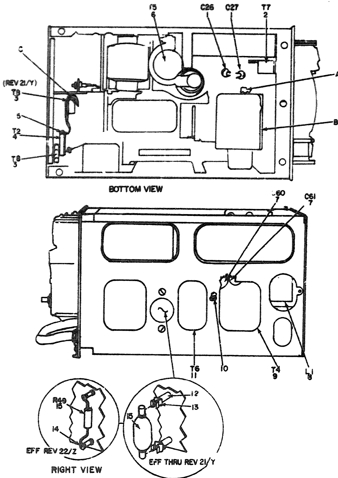
Figure 20. Receiver-Transmitter, Radio RT-711/APN-158, Additional Parts Location (Sheet 1 of 4).
