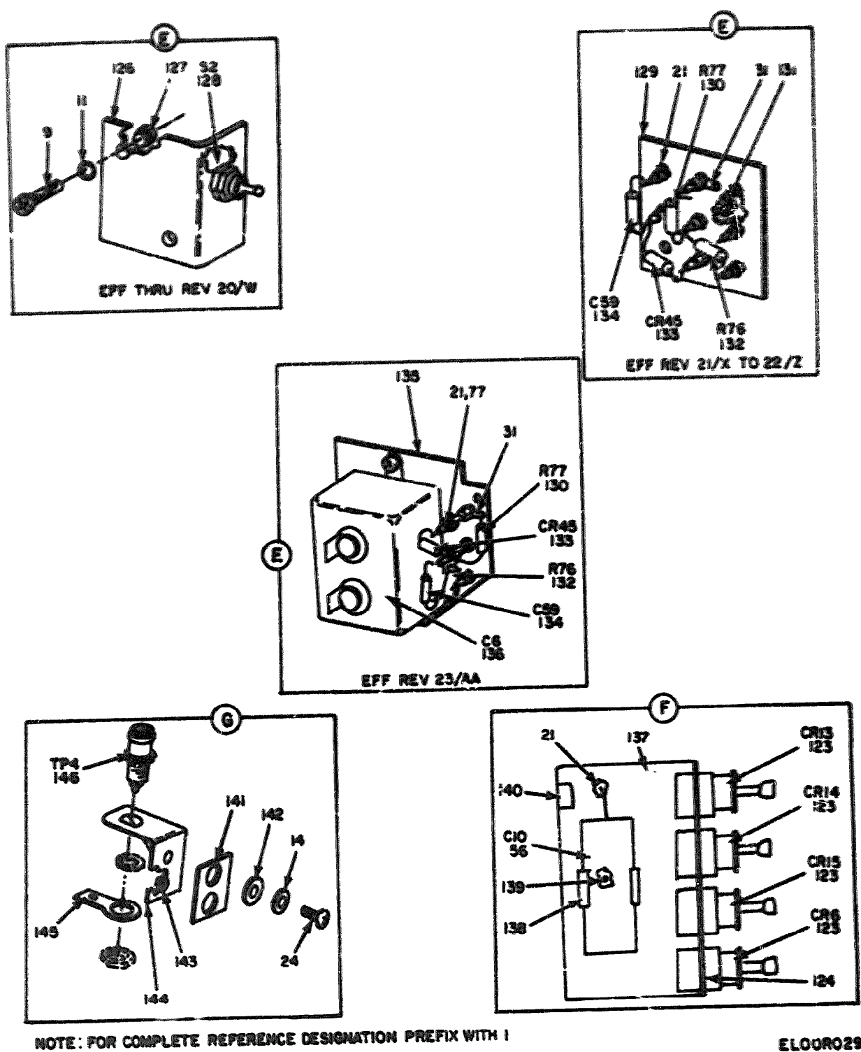
Figure 19. Receiver-Transmitter, Radio RT-711/APN-158, Parts Location (Sheet 4 of 4).
