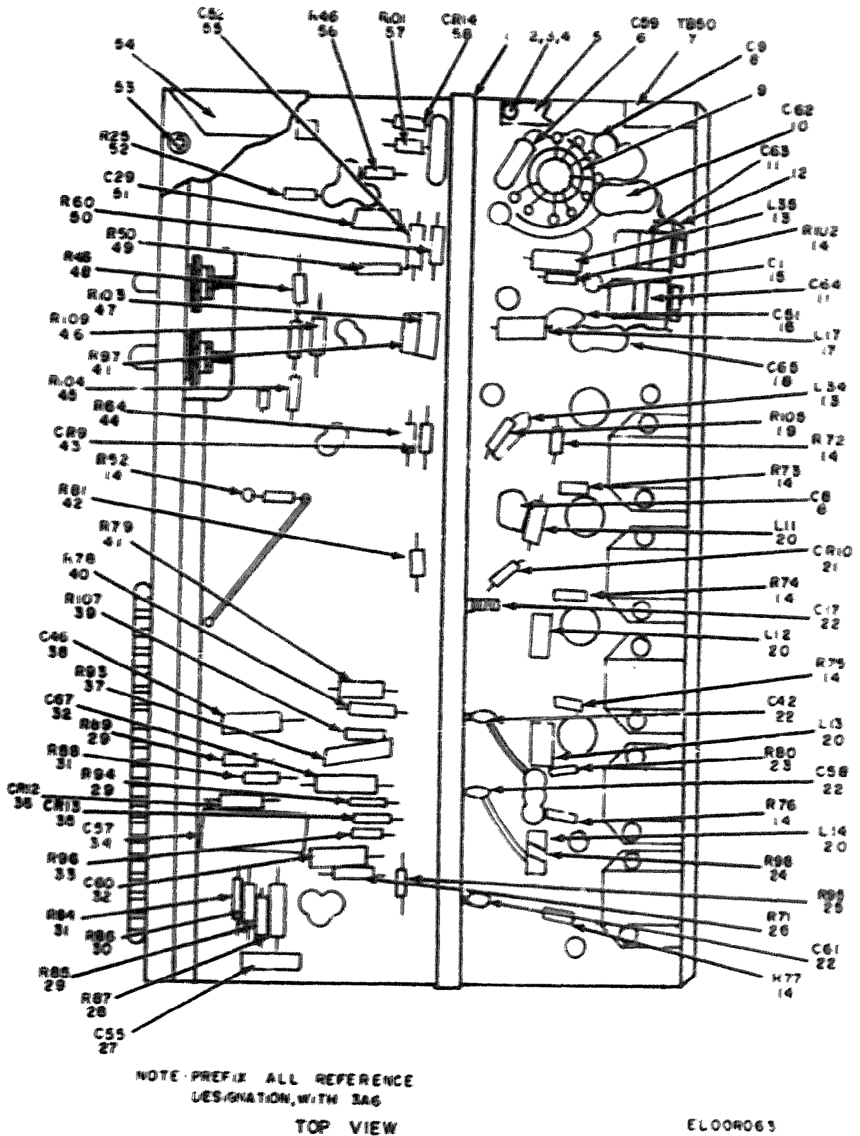
Figure 46. If Amplifier Assembly (3A6) (Sheet 1 of 3).
