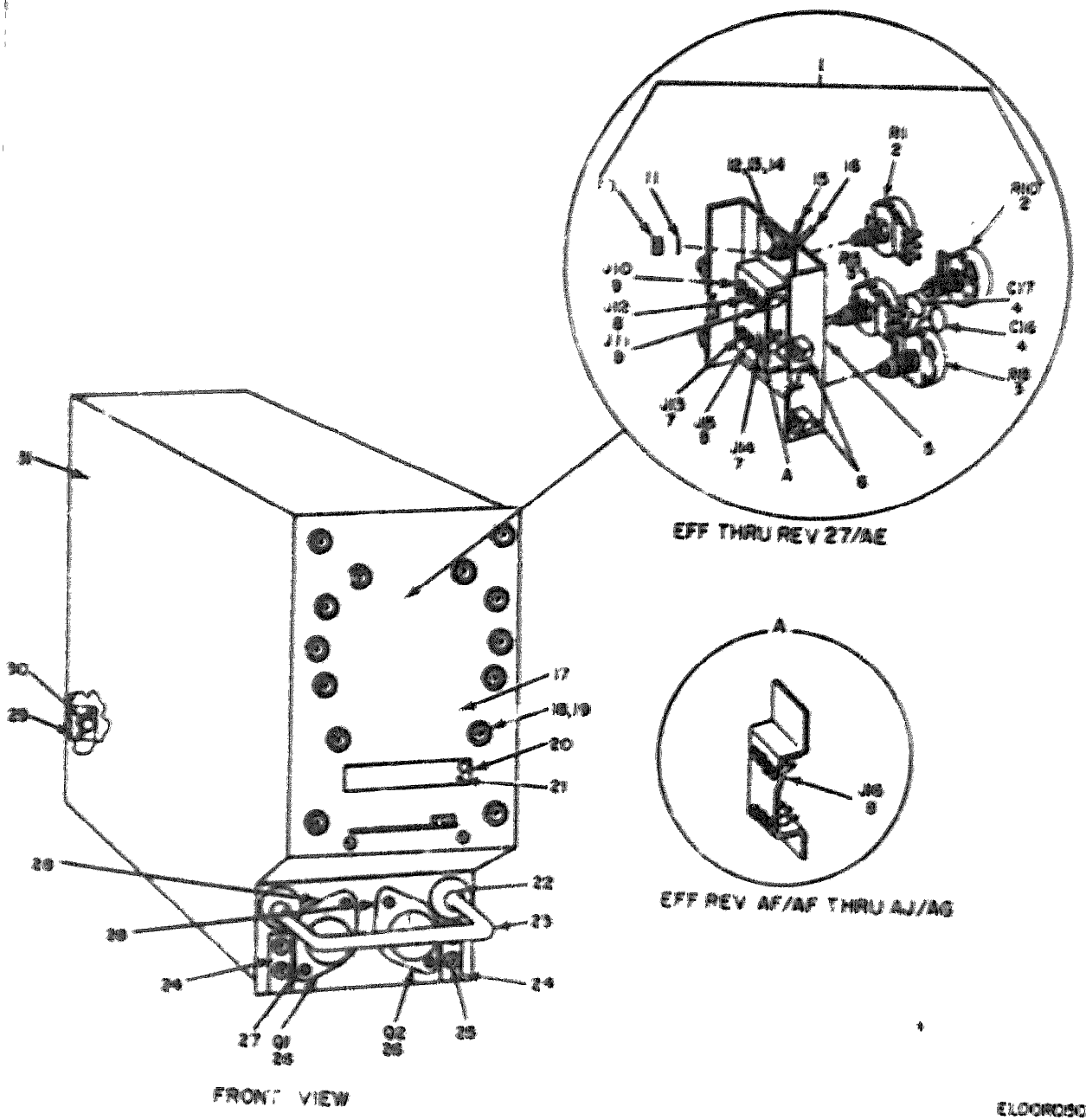
Figure 37. Synchronizer, Electrical SM-358/APN-158 (Sheet 1 of 2).
