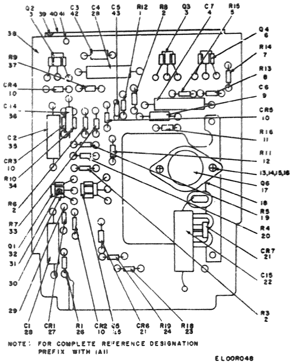
Figure 35. Wired Trigger Generator (1A11) (564-2103-004 Rev H/H).
