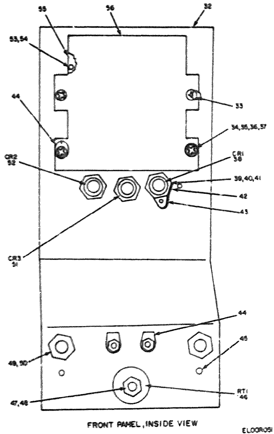
Figure 37. Synchronizer, Electric SN-358/APN-158 (Sheet 2 of 2).
