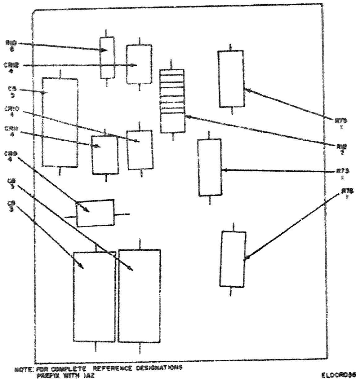
Figure 23. Power Supply (1A2) (556-9558-004).
