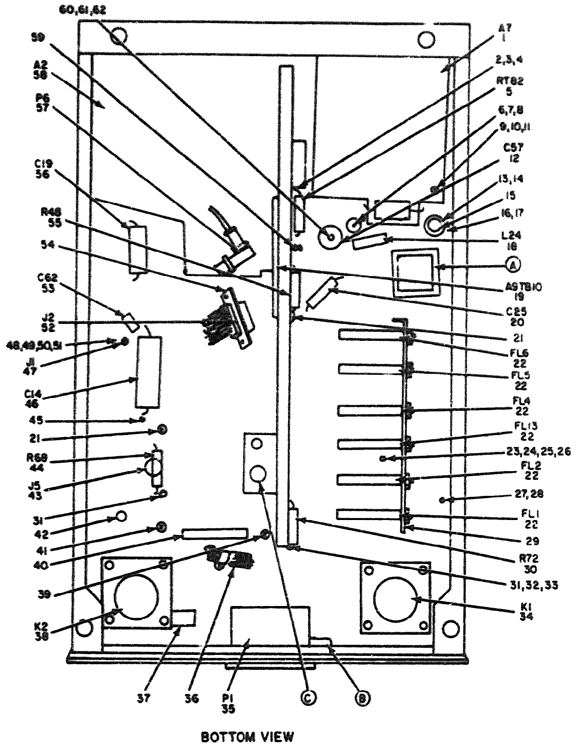
Figure 19. Receiver-Transmitter, Radio RT-711/APN-158, Parts Location (Sheet 1 of 4).
