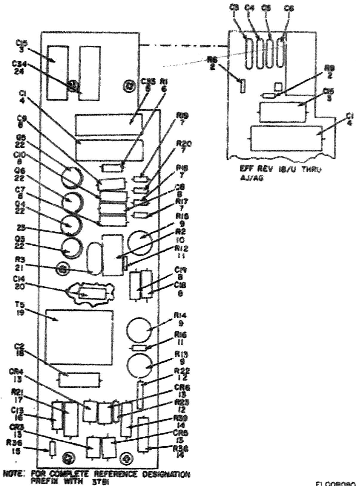
Figure 55. Detector Board Assembly (3TB1) (556-9552-003 and 556-9552-006).
