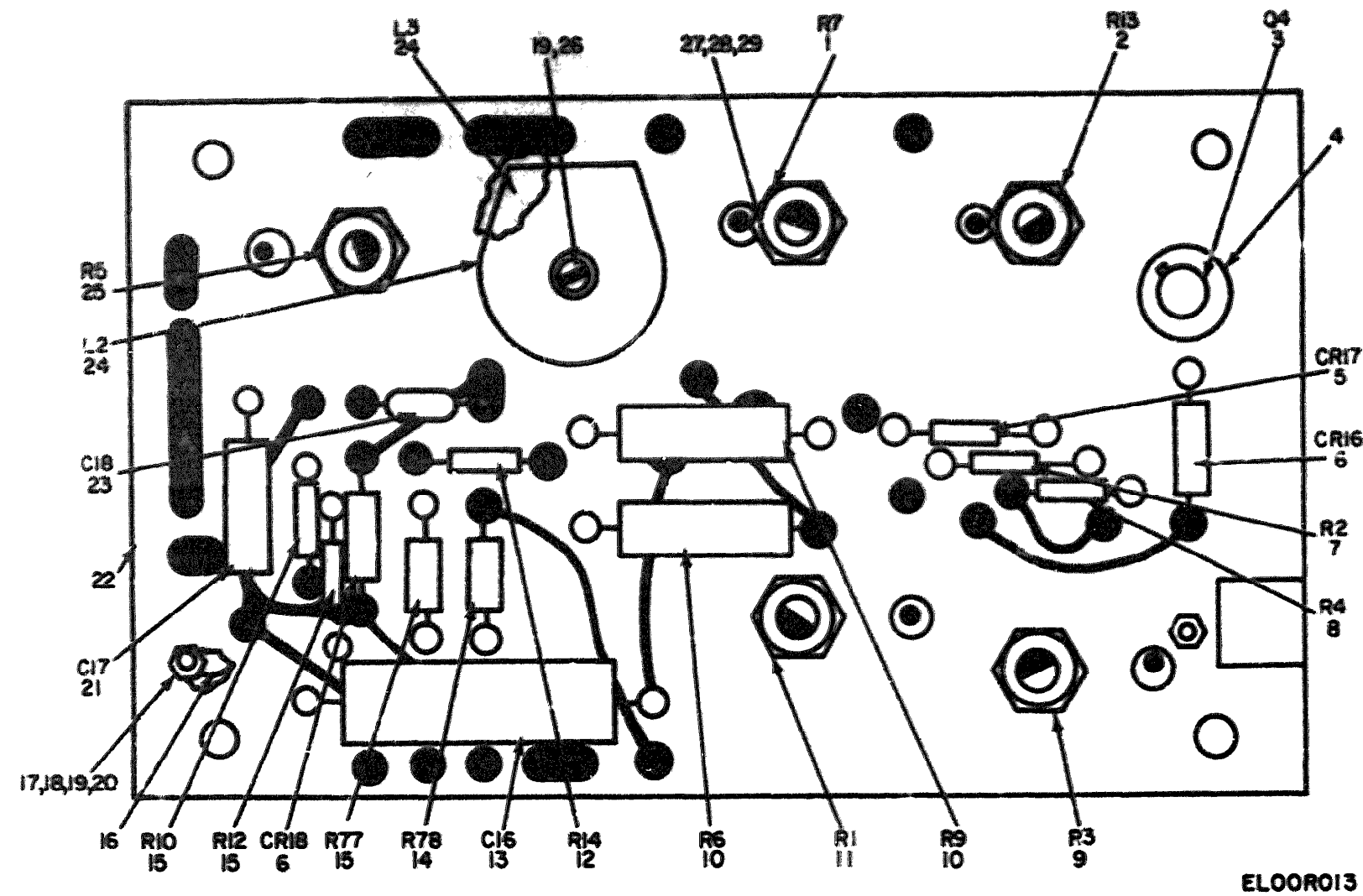
Figure 10. Terminal Board (TB1).
