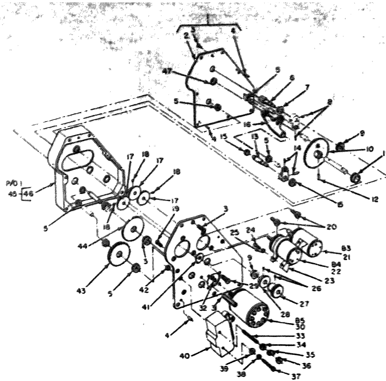
Figure 3. Geartrain Assembly (563-5724-005).
