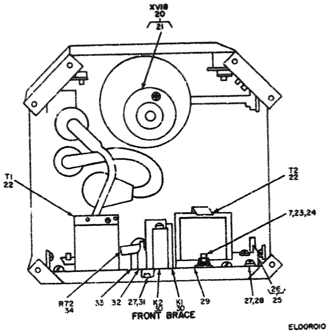
Figure 8. Chassis, Indicator Assembly (Sheet 2 of 2).
