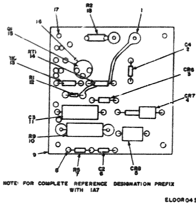
Figure 30. Circuit Card Assembly, Fault Sensing (1A7) (564-2109-003 Rev J).
