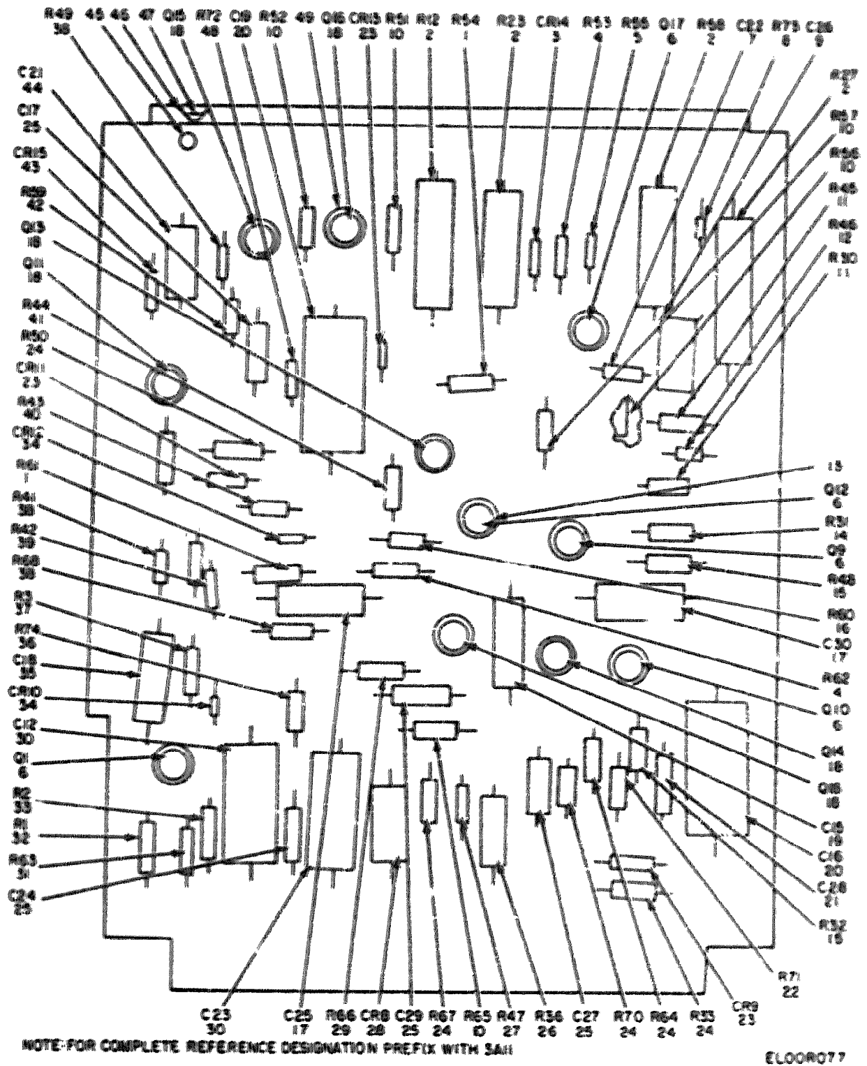
Figure 53. Video Drive Assembly (3A11) (757-0719-003).
