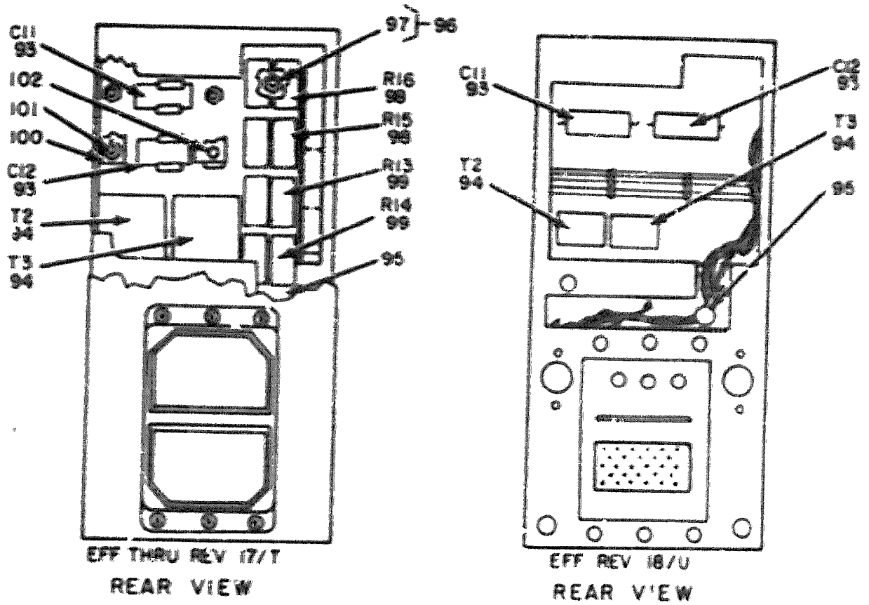
Figure 38. Synchronizer, Electrical SN-358/APN-158, Additional Parts Location (Sheet 4 of 4).
