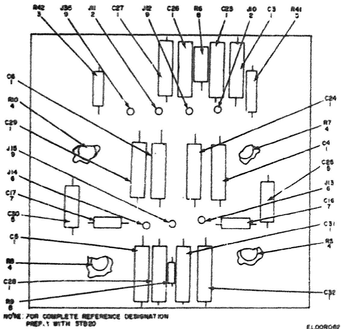
Figure 57. Board Assembly (37820).
