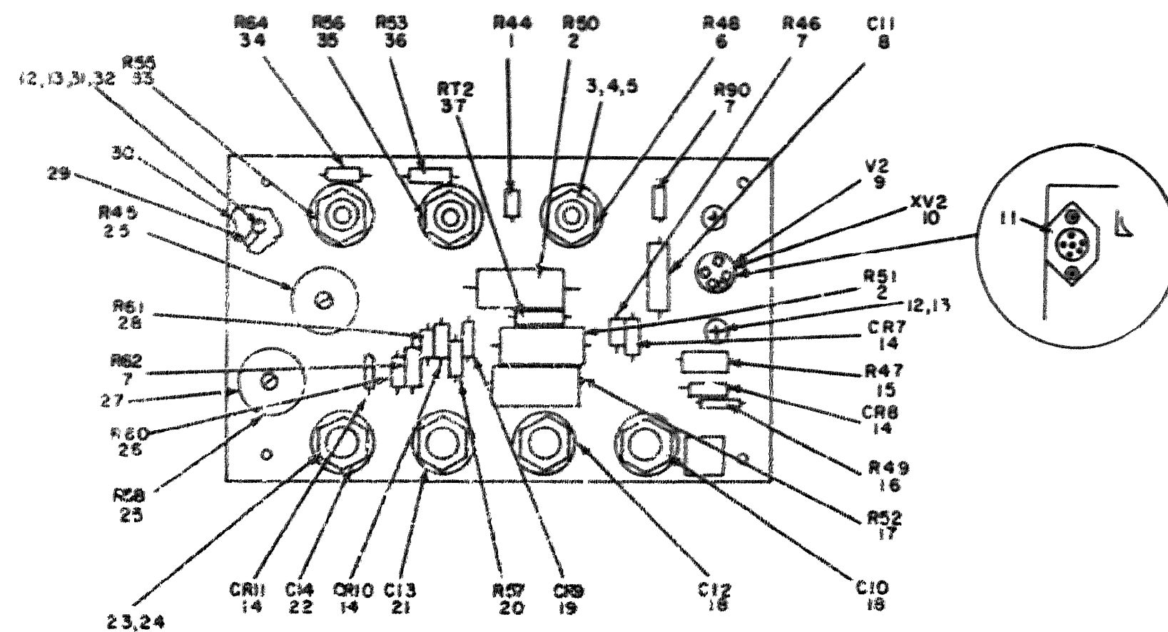
Figure 13. Terminal Board (TB3).
