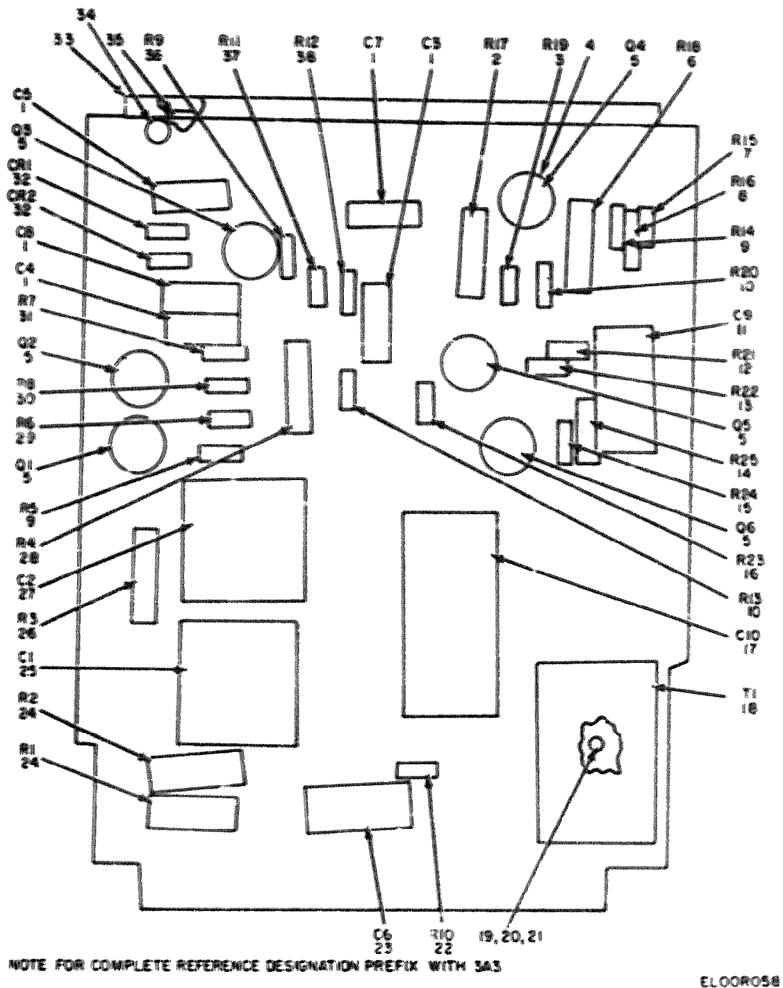
Figure 41. Amplifier, Servo Elevations (3A3) (769-7195-001).
