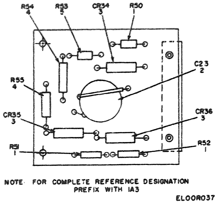
Figure 24. Keep Alive Supply (1A3).
