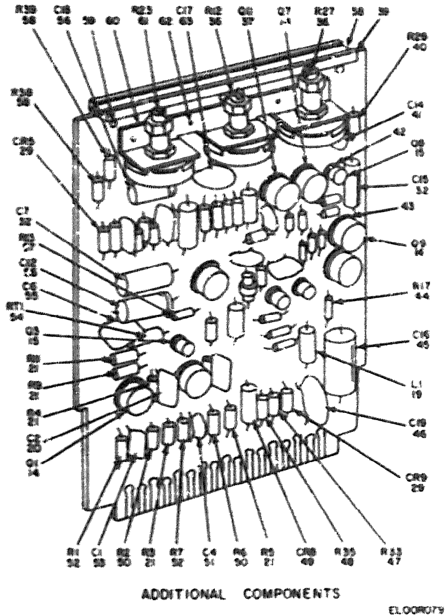
Figure 54. Video Drive Assembly (3A11) (565-5407-005) (Sheet 2 of 2).
