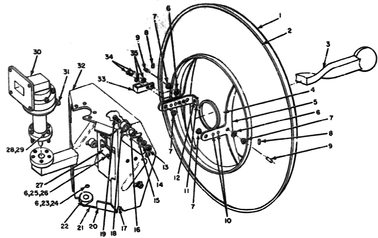
Figure 5. Gimbal Assembly.
