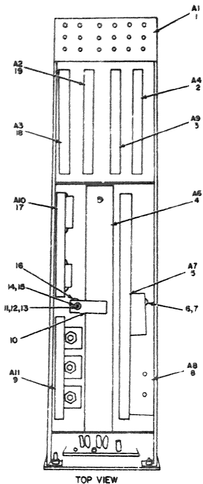
Figure 38. Synchronizer, Electrical SN-358/APN-158, Additional Parts Location (Sheet 1 of 4).
