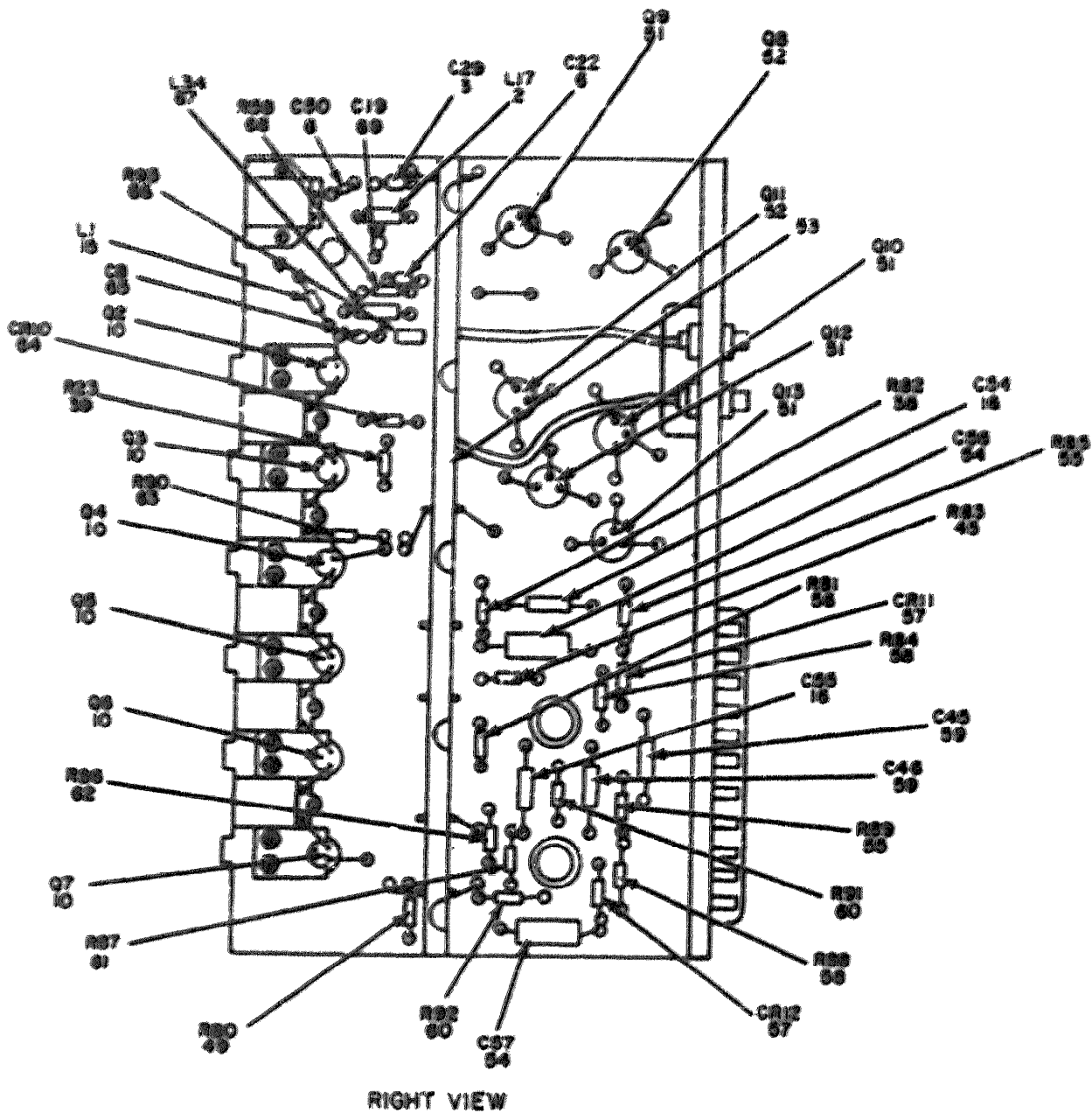
Figure 47. If Amplifier Assembly (3A6) Additional Parts Location (Sheet 3 of 5).
