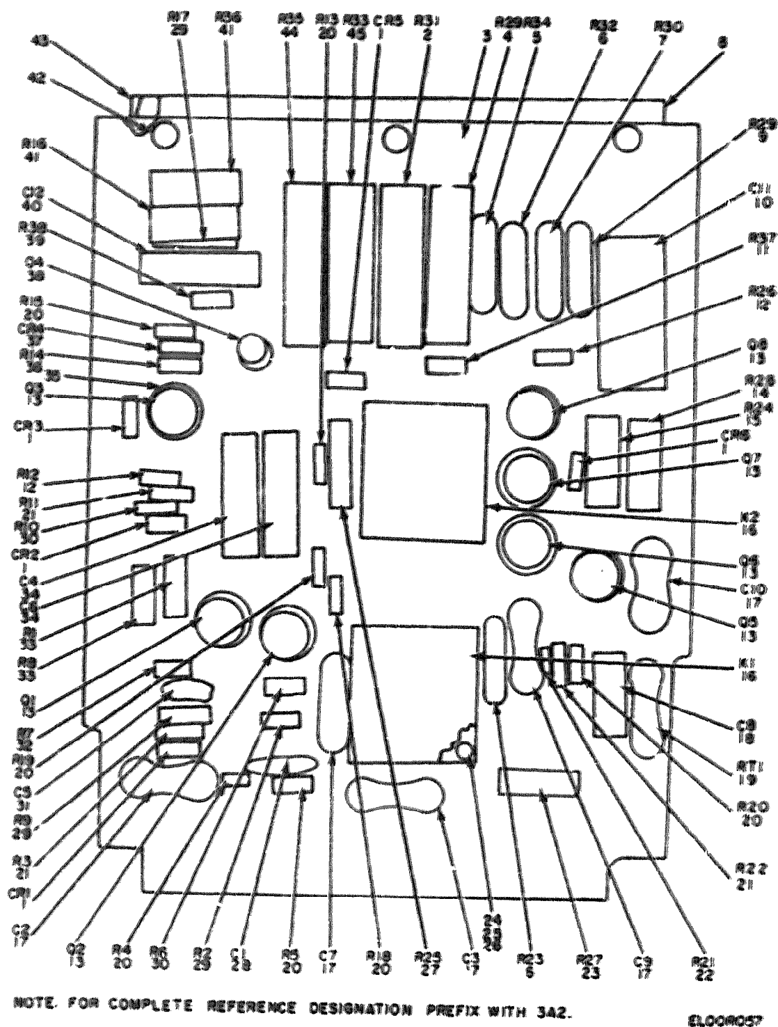
Figure 40. Gate Generator Board Assembly (3A2).
