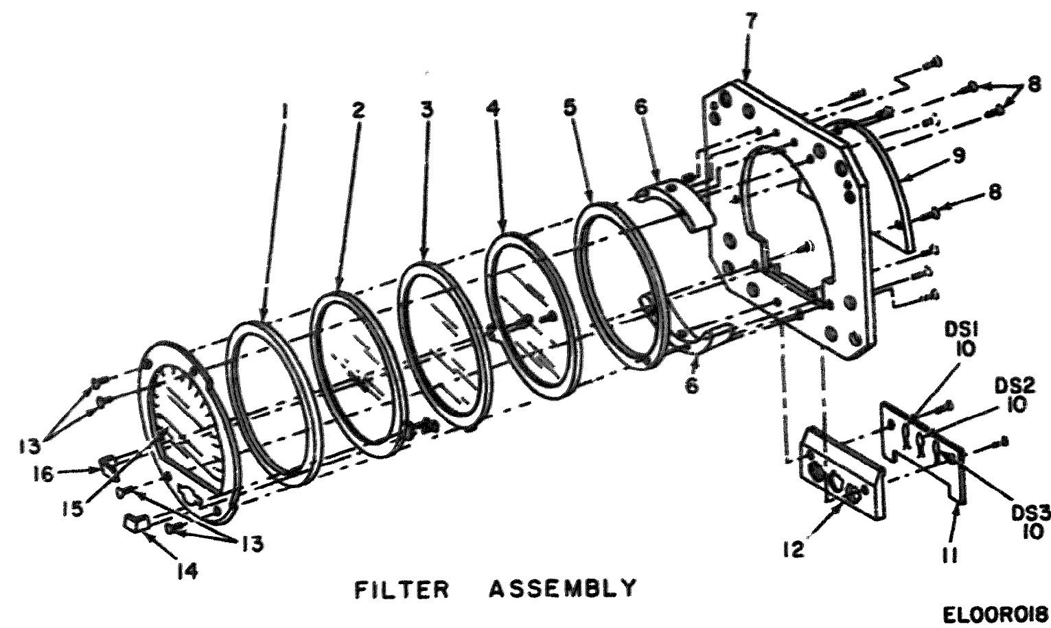
Figure 15. Filter Assembly (Sheet 1 of 2).
