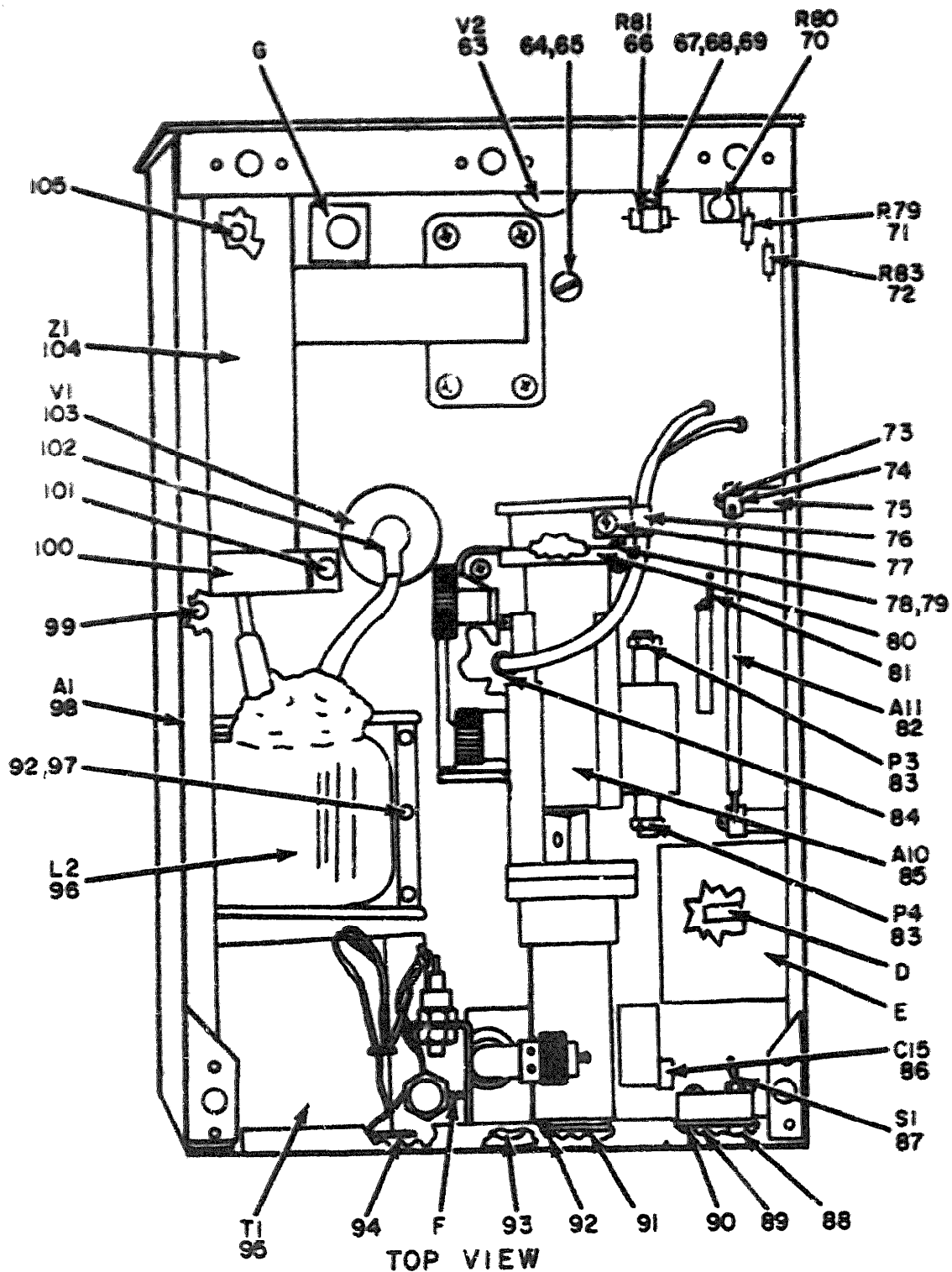
Figure 19. Receiver-Transmitter, Radio RT-711/APN-158, Parts Location (Sheet 2 of 4).
