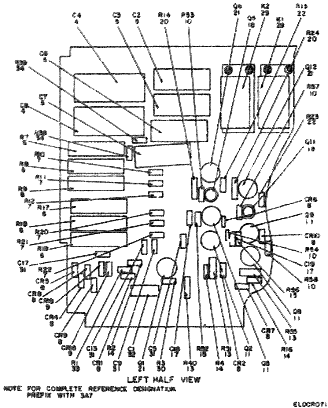
Figure 48. Generator-Amplifier, Sweep (3A7) (Sheet 2 of 3).
