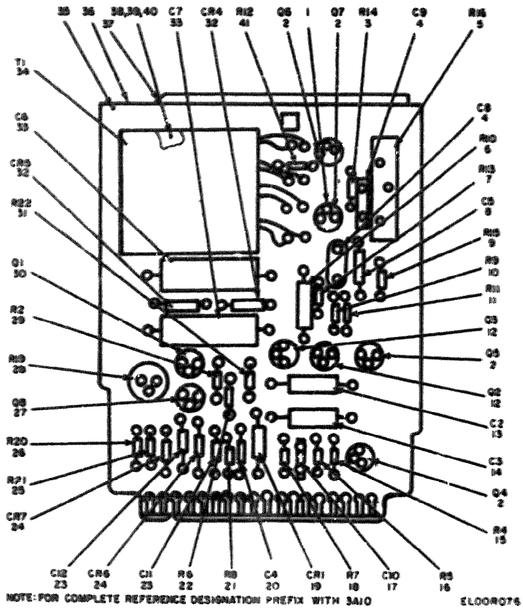
Figure 52. AFC Assembly (3A10) (758-4825-001).
