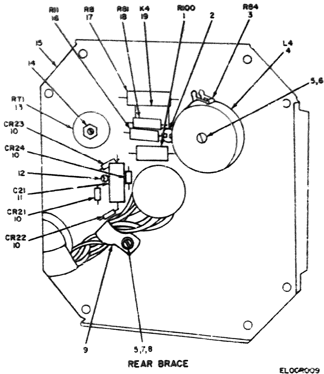
Figure 8. Chassis, Indicator, Assembly (Sheet 1 of 2).
