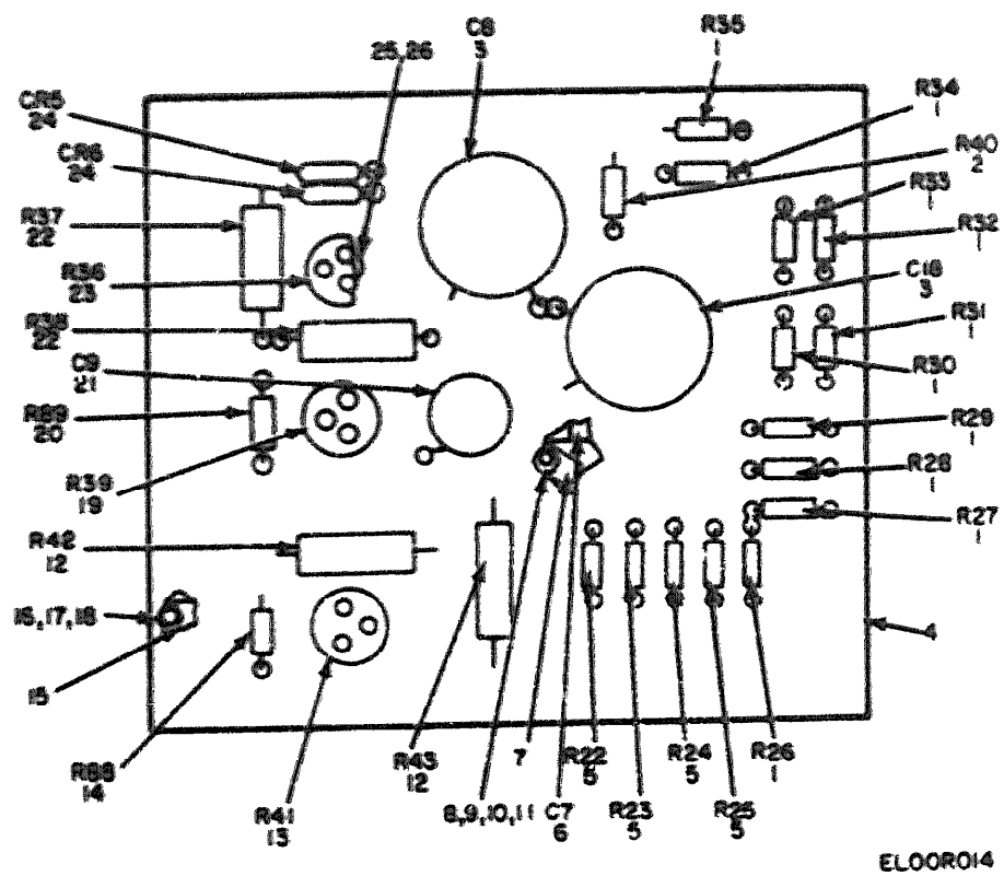
Figure 11. Terminal Board (TB2) (565-5548-004).
