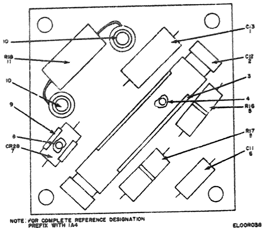
Figure 25. Wired Minus 27.5V Regulator (1A4).
