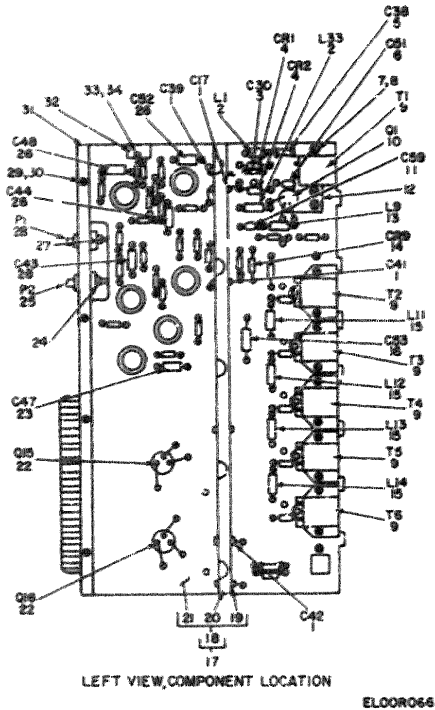
Figure 47. If Amplifier Assembly (3A6) Additional Parts Location (Sheet 1 of 4).
