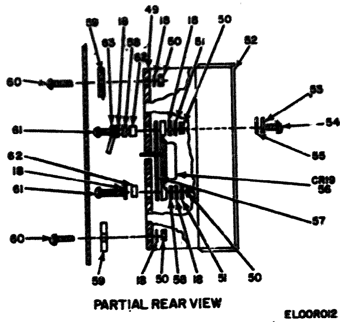
Figure 9. Chassis, Indicator Assembly, Exploded View (Sheet 2 of 2).
