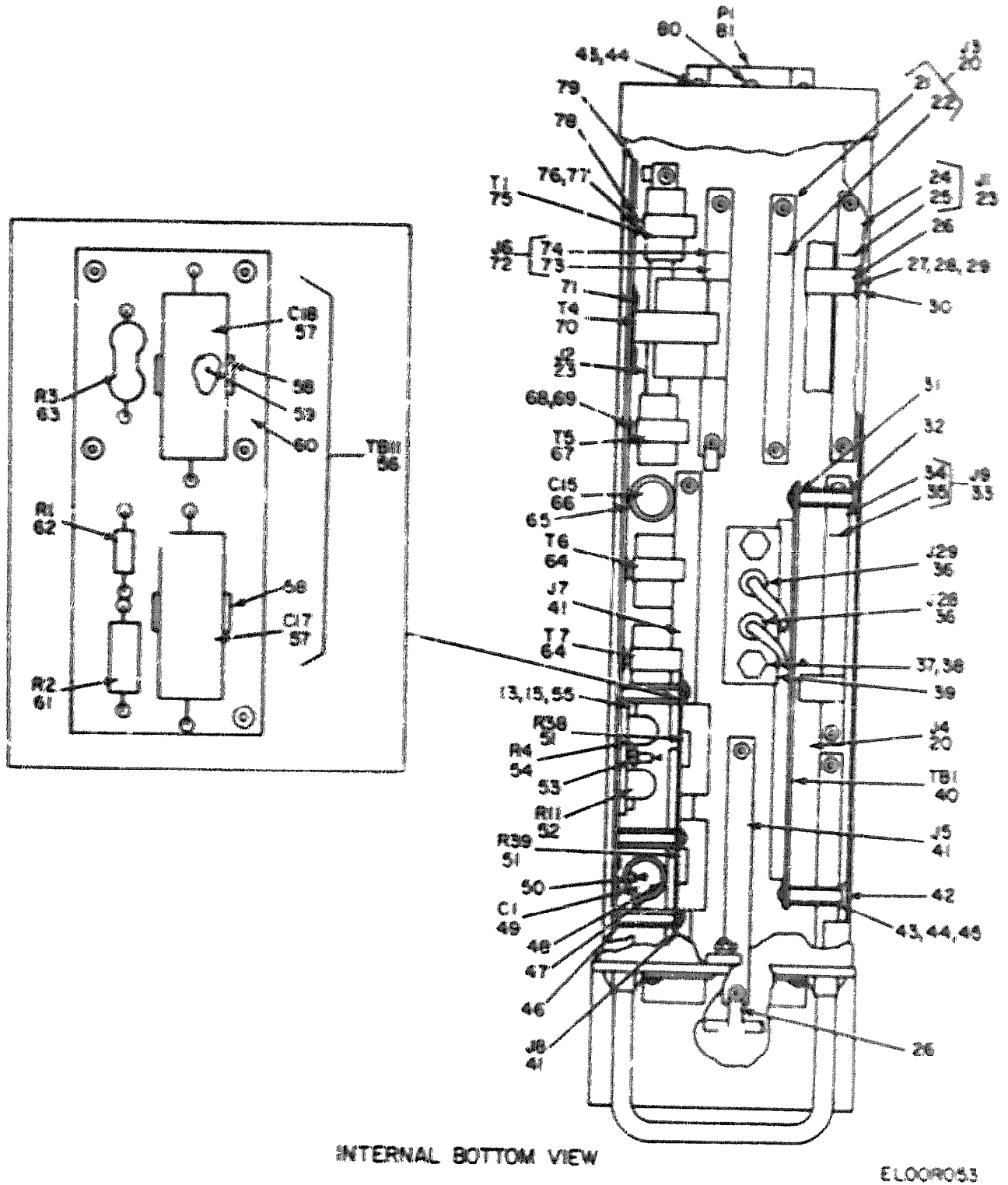
Figure 38. Synchronizer, Electrical SN-358/APN-158, Additional Parts Location (Sheet 2 of 4).
