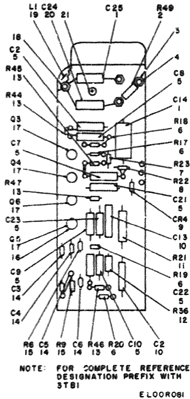
Figure 56. Detector Board Assembly (3TB1) (565-5621-004).
