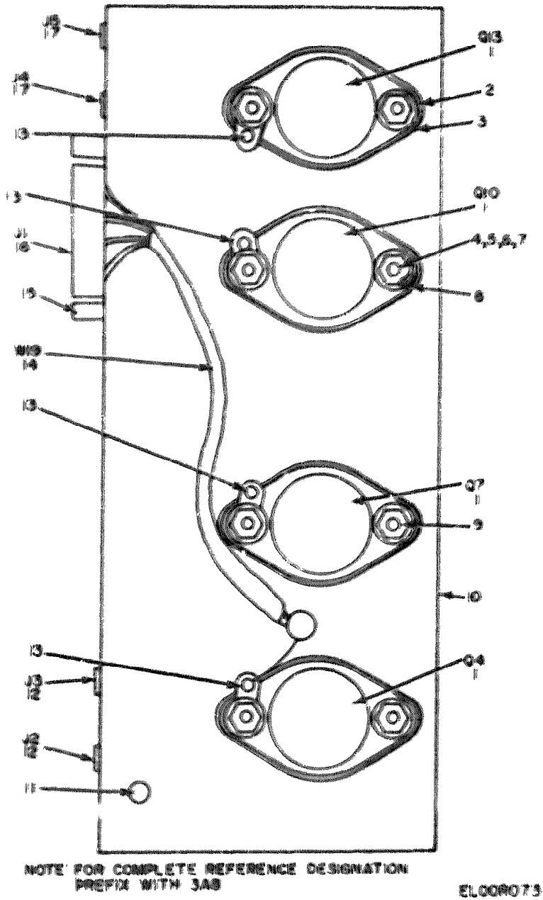
Figure 49. Heatsink Assembly (3A8).
