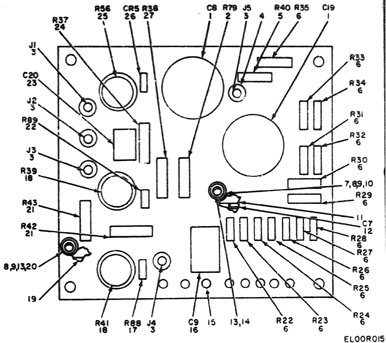
Figure 12. Terminal Board (TB2) (758-0336-001).
