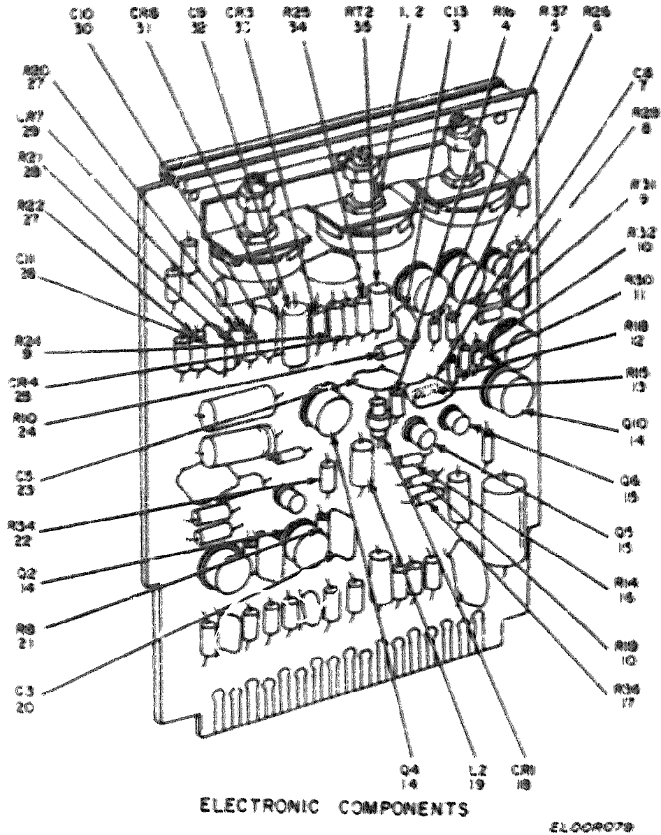
Figure 54. Video Drive Assembly (3A11) (565-5607-005) (Sheet 1 of 2).
