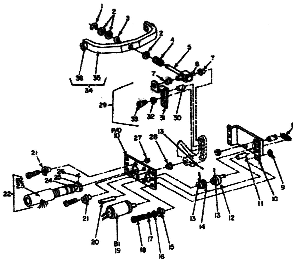
Figure 4. Geartrain Assembly (563-4848-003).
