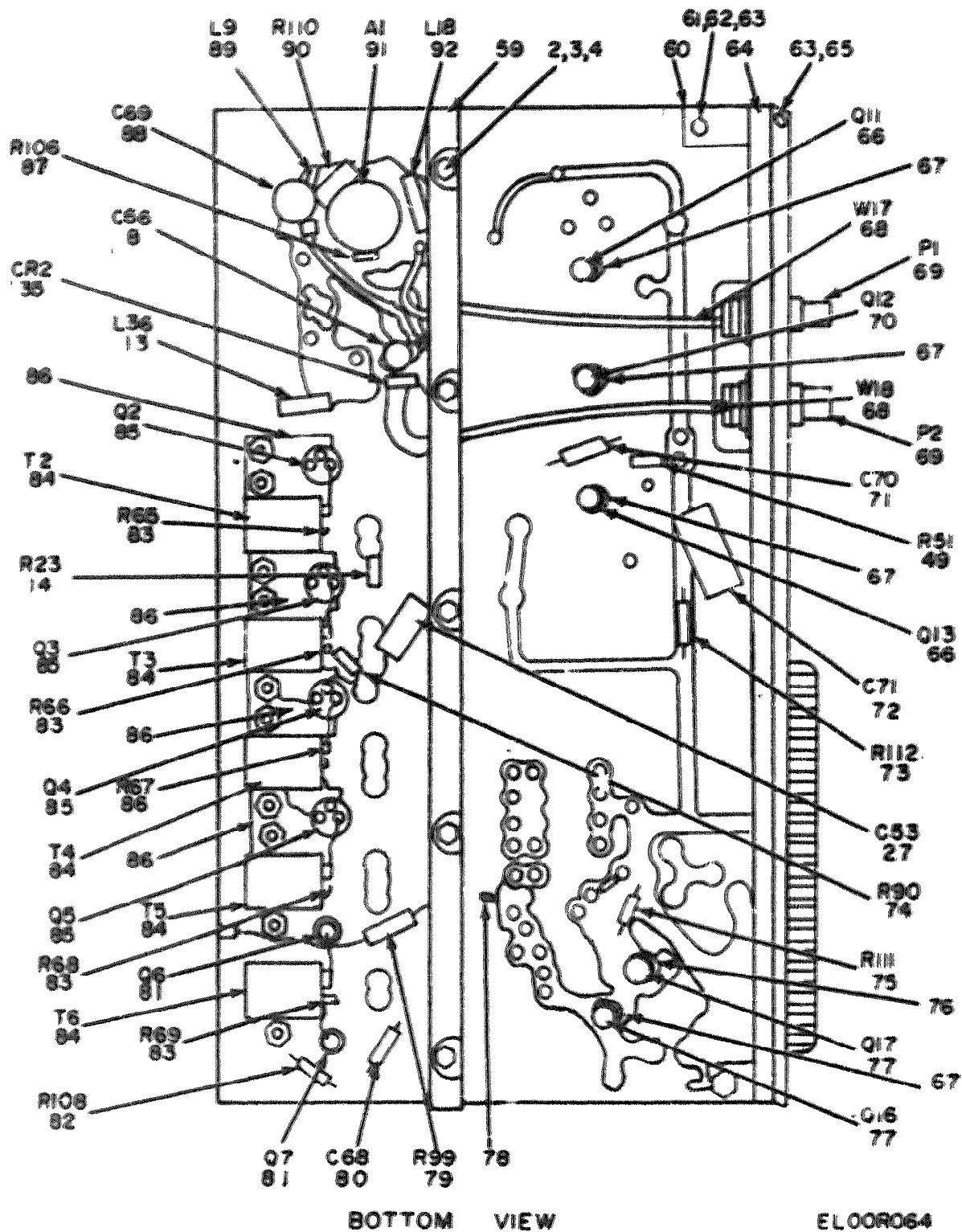
Figure 46. If Amplifier Assembly (3A6) (Sheet 2 of 3).
