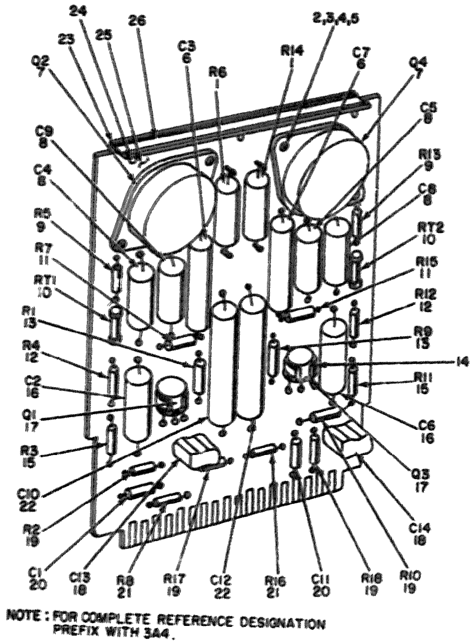
Figure 45. Isolation Amplifier Assembly (3A4) (566-0050-004).
