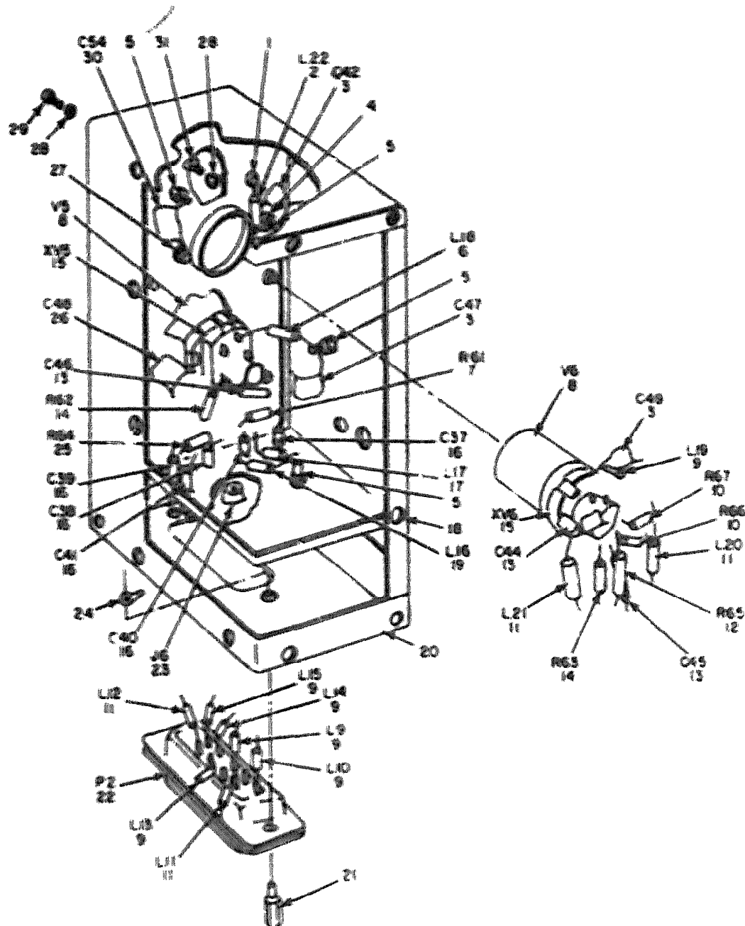
Figure 33. Preamplifier Assembly (1A10A1).
