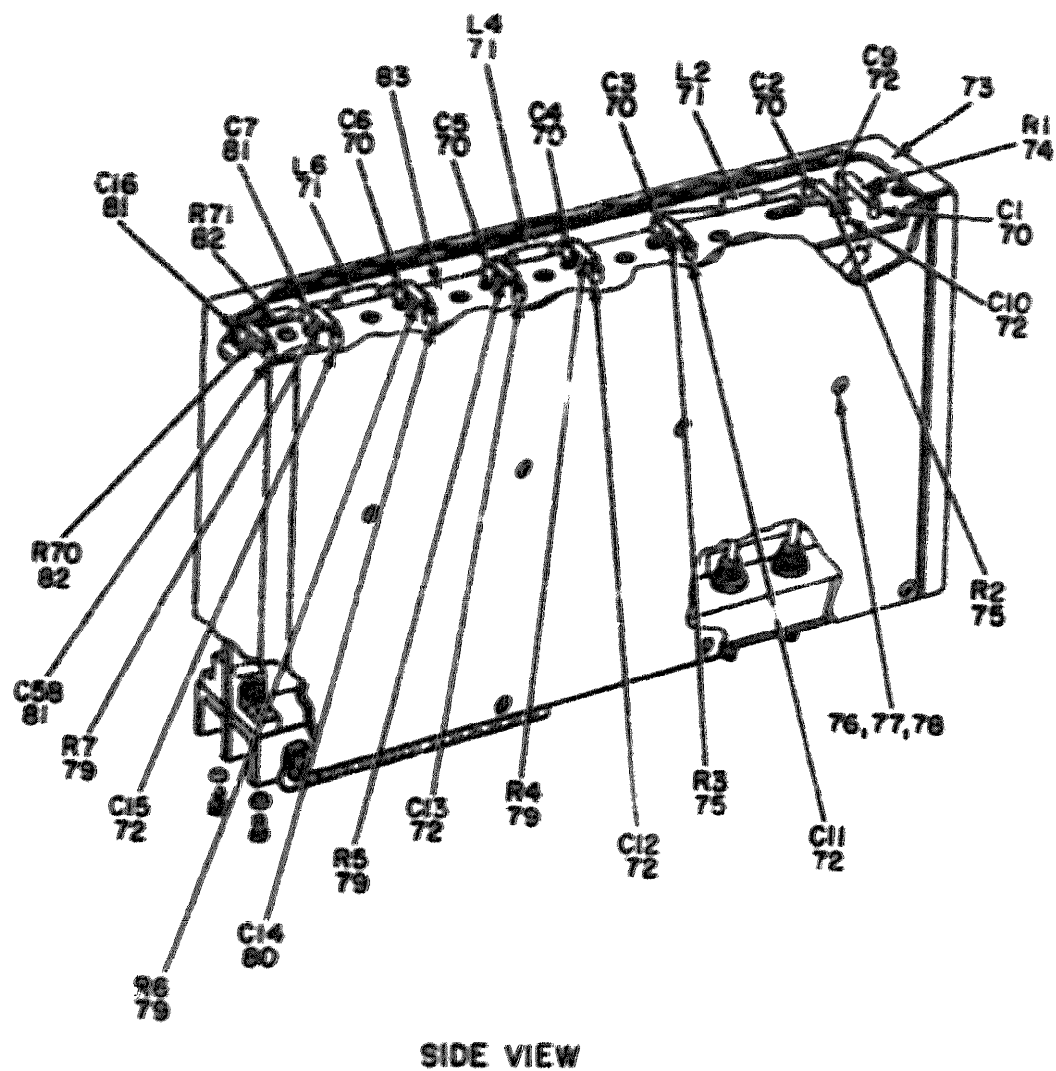
Figure 47. If Amplifier Assembly (3A6) Additional Parts Location (Sheet 4 of 4).
