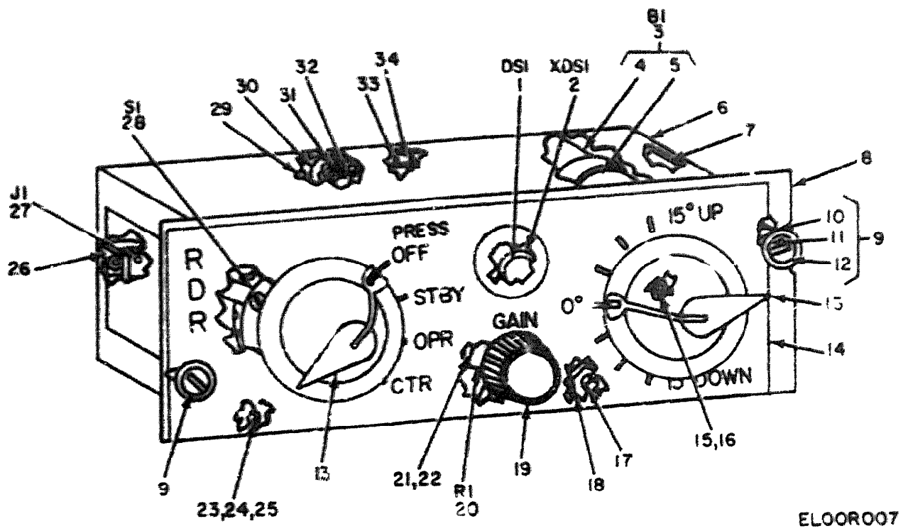
Figure 6. Control, Radar Set C-4881/APN-158.
