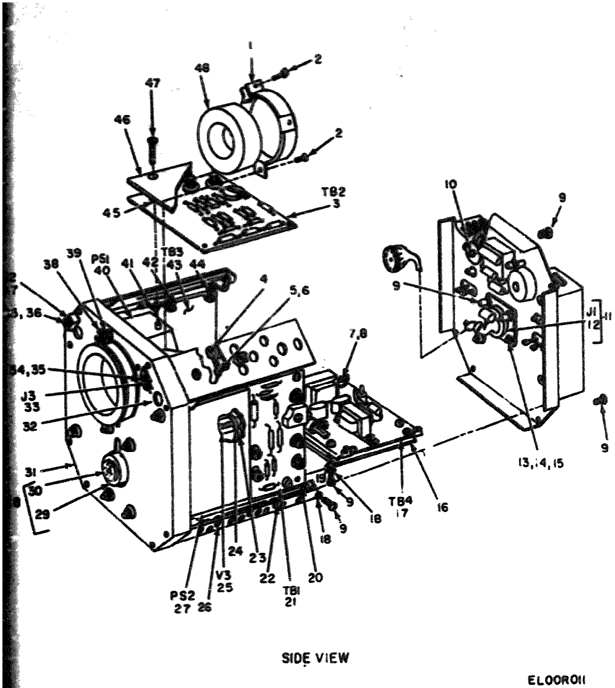
Figure 9. Chassis, Indicator Assembly Exploded View (Sheet 1 of 2).
